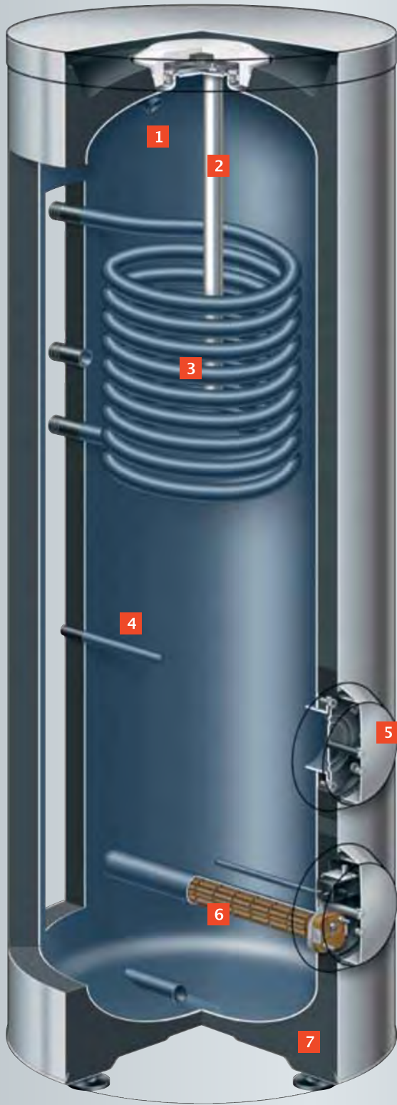
Vitocell 100-B (Modelo CVE)
